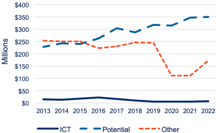
PA-9 Services Exports, 2013-2022
